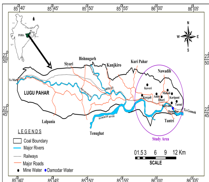
Figure 1. Map of the East Bokaro Coalfield showing the sampling locations.
